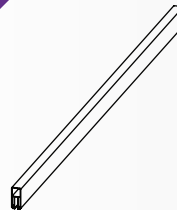
Top Rail (1) 1\frac{1}{2} " x 3\frac{1}{2} " x 81\frac{1}{2} "
