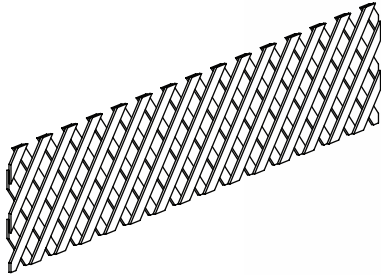
Lattice Section (1) \frac{1}{2} " x 12" x 81\frac{1}{4} "
