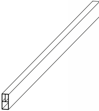
Top Rail (1) 1½" x 3½" x 81½"
