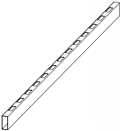
Top Rail (1) 1½" x 3½" x 81½"
