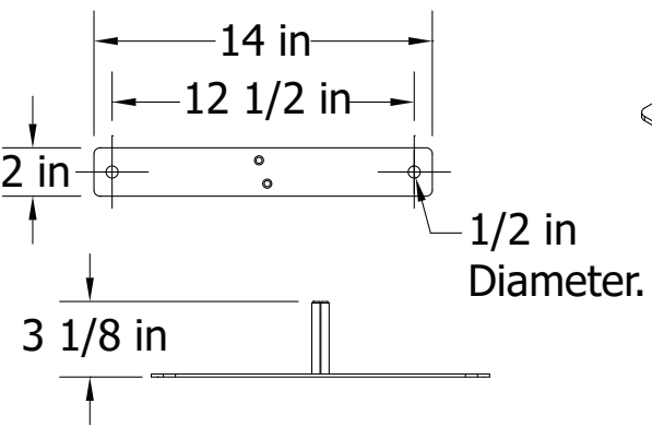
Metal Feet
