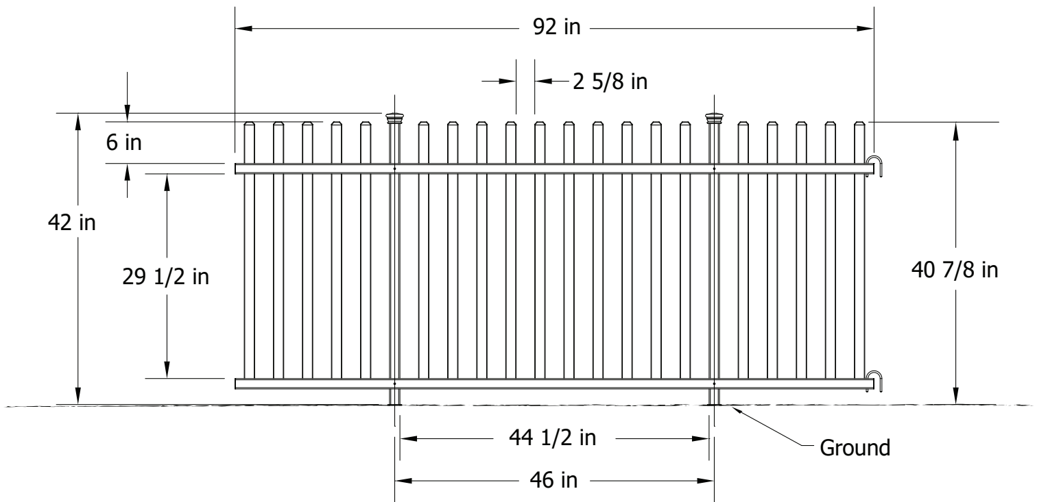
Metal Feet
