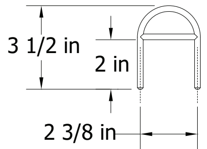
Metal U-Joiner
